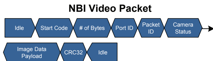
Figure 12 – NBI Video Packet
