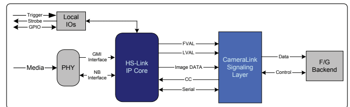
Figure 2 – Topology of HSLink from a Framegrabber perspective
