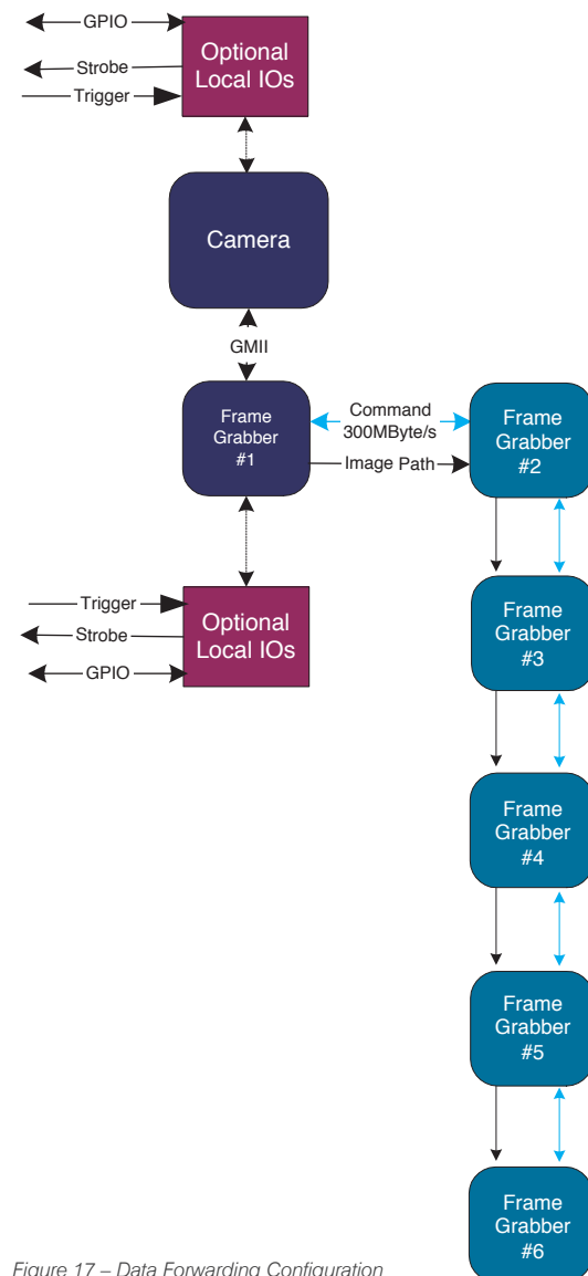
Figure 17 – Data Forwarding Configuration
