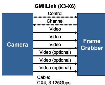
Figure 4 – GMILink Configuration
