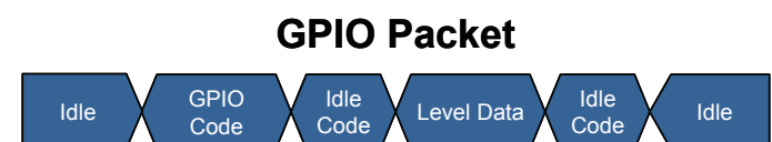
Figure 10 – GPIO Packet
