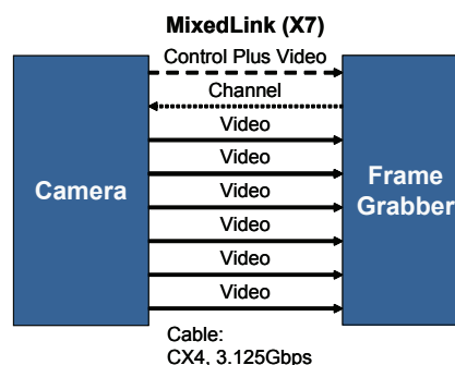
Figure 6 – MixedLink configuration
