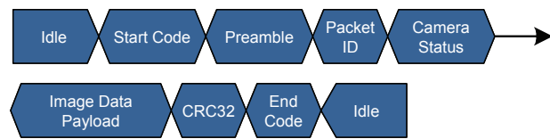
Figure 13 – GMII Video Packet
