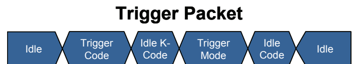
Figure 9 – Trigger Packet
