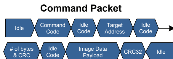
Figure 14 – Command Packet
