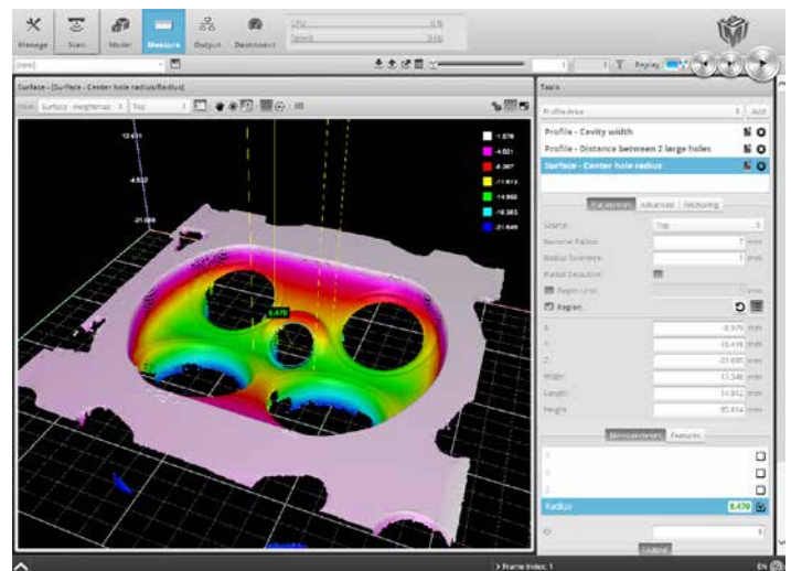
Gocator's browser-based graphical user interface showing the scan coverage of an automotive cylinder head
